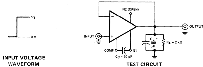
FIGURE 1—RISE TIME, OVERSHOOT, AND SLEW RATE
