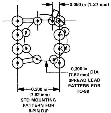
0.300-DIAMETER SPREAD LEAD CIRCLE FOR TO-99
