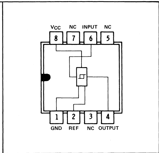
JG OR P DUAL-IN-LINE PACKAGE (TOP VIEW)
