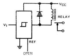
FIGURE 10—RELAY DRIVER
