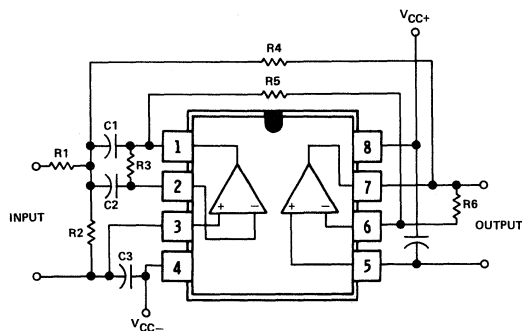
MULTIPLE-FEEDBACK ACTIVE BANDPASS FILTER
