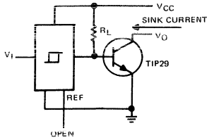
FIGURE 8—EXTERNAL N-P-N TRANSISTOR FOR INCREASING SINK CURRENT
