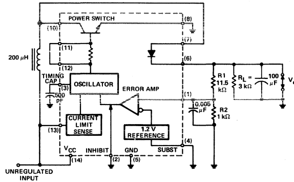
FIGURE 1—TEST CIRCUIT
