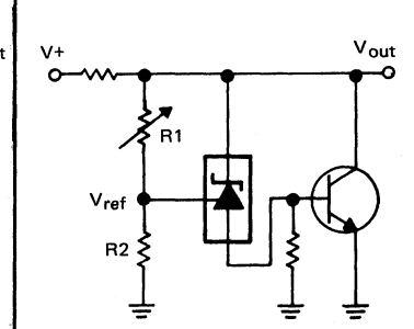
FIGURE 7—CROW BAR
