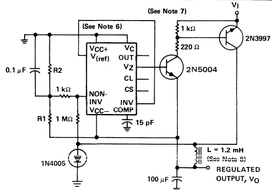
FIGURE 10—NEGATIVE SWITCHING REGULATOR
