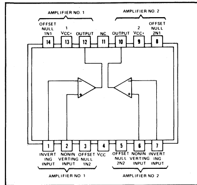
L PLUG-IN PACKAGE (TOP VIEW)
