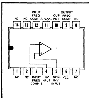
J OR N DUAL-IN-LINE PACKAGE (TOP VIEW)
