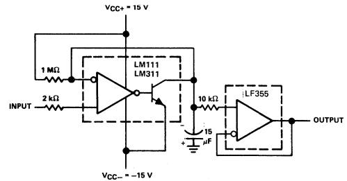
FIGURE 25— NEGATIVE-PEAK DETECTOR
