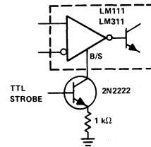
FIGURE 13—STROBING
