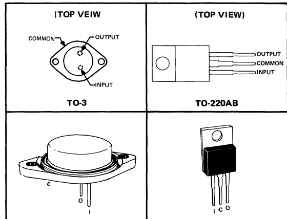
KA PACKAGE
