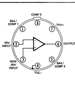
L PLUG-IN PACKAGE (TOP VIEW)
