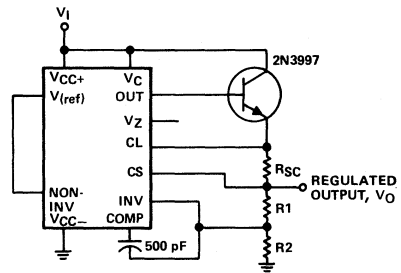
FIGURE 4—POSITIVE VOLTAGE REGULATOR (EXTERNAL N-P-N PASS TRANSISTOR)
