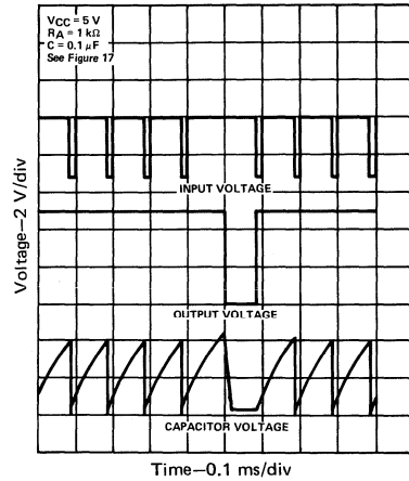
FIGURE 18—MISSING-PULSE-DETECTOR WAVEFORMS
