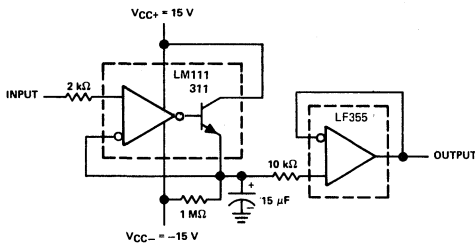
FIGURE 24— POSITIVE-PEAK DETECTOR
