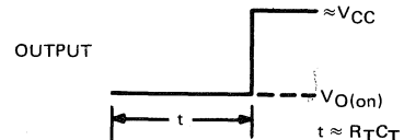
FIGURE 7—BASIC TIMED-INTERVAL CIRCUIT
