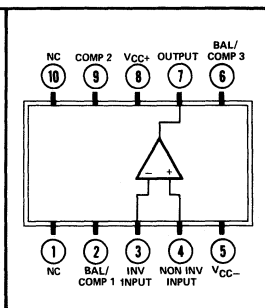
U FLAT PACKAGE (TOP VIEW)
