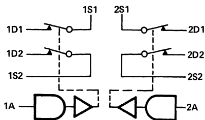
schematic (each channel)
