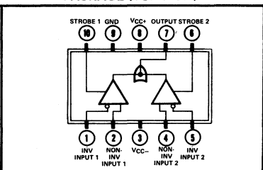
U FLAT PACKAGE (TOP VIEW)
