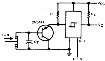
FIGURE 11—LONG-TIMED-INTERVAL CIRCUIT
