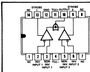
J OR N DUAL-IN-LINE PACKAGE (TOP VIEW)
