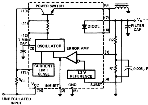
FIGURE 4—NEGATIVE REGULATOR (e.g., +5 VOLTS INPUT TO -5 VOLTS OUTPUT) OR (i.e., POSITIVE INPUT, NEGATIVE OUTPUT)
