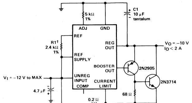
FIGURE 2—HIGH-CURRENT REGULATOR
