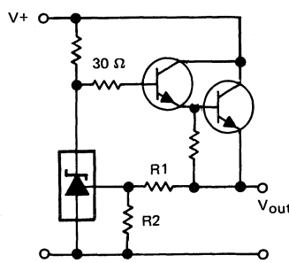
FIGURE 6—SERIES REGULATOR
