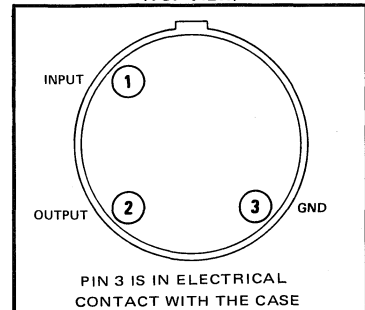
LA PLUG-IN PACKAGE (TOP VIEW)
