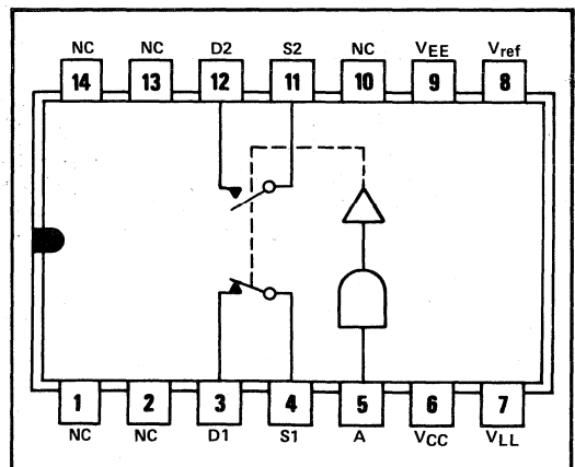
N DUAL-IN-LINE PACKAGE (TOP VIEW)
