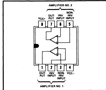
L PLUG-IN PACKAGE (TOP VIEW)
