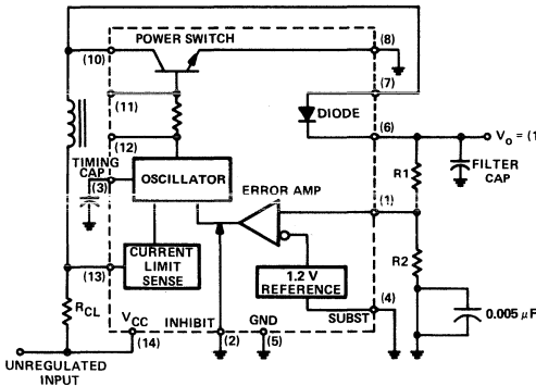
FIGURE 2—POSITIVE REGULATOR, STEP-UP CONFIGURATION
