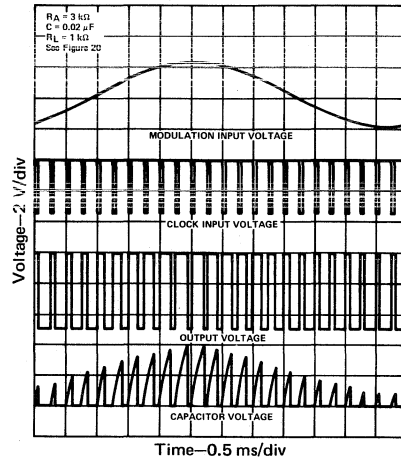
FIGURE 21—PULSE-WIDTH-MODULATION WAVEFORMS
