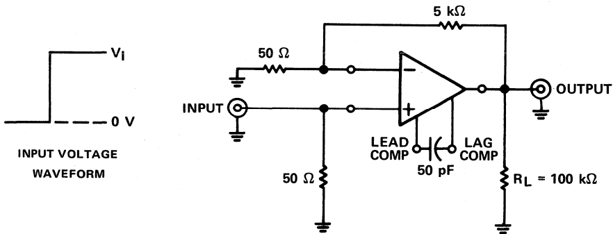
FIGURE 2—GAIN-OF-100 AMPLIFIER
