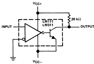
FIGURE 14—ZERO-CROSSING DETECTOR
