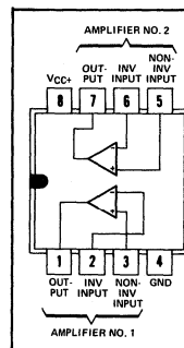
JG OR P DUAL-IN-LINE PACKAGE (TOP VIEW)
