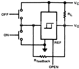
FIGURE 11—LONG-TIMED-INTERVAL CIRCUIT
