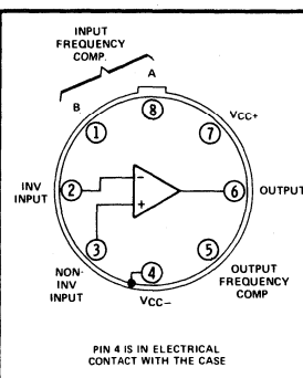
L PLUG-IN PACKAGE (TOP VIEW)
