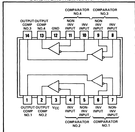
DUAL-IN-LINE PACKAGE (TOP VIEW)
