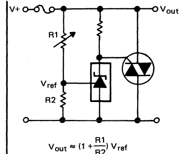
FIGURE 7—CROW BAR
