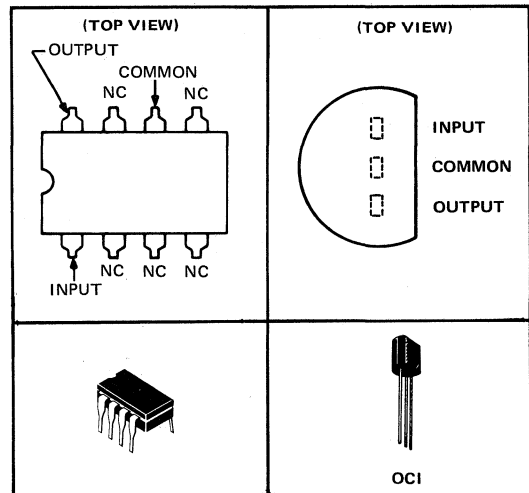
JG DUAL-IN-LINE PACKAGE
