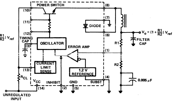
FIGURE 3—POSITIVE REGULATOR, STEP-DOWN CONFIGURATION
