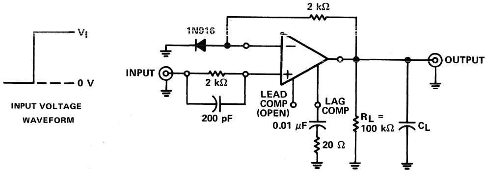
FIGURE 1—UNITY-GAIN AMPLIFIER
