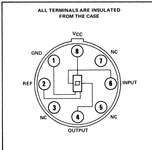
L PLUG-IN PACKAGE (TOP VIEW)
