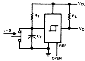
FIGURE 12—BOUNCELESS SWITCH
