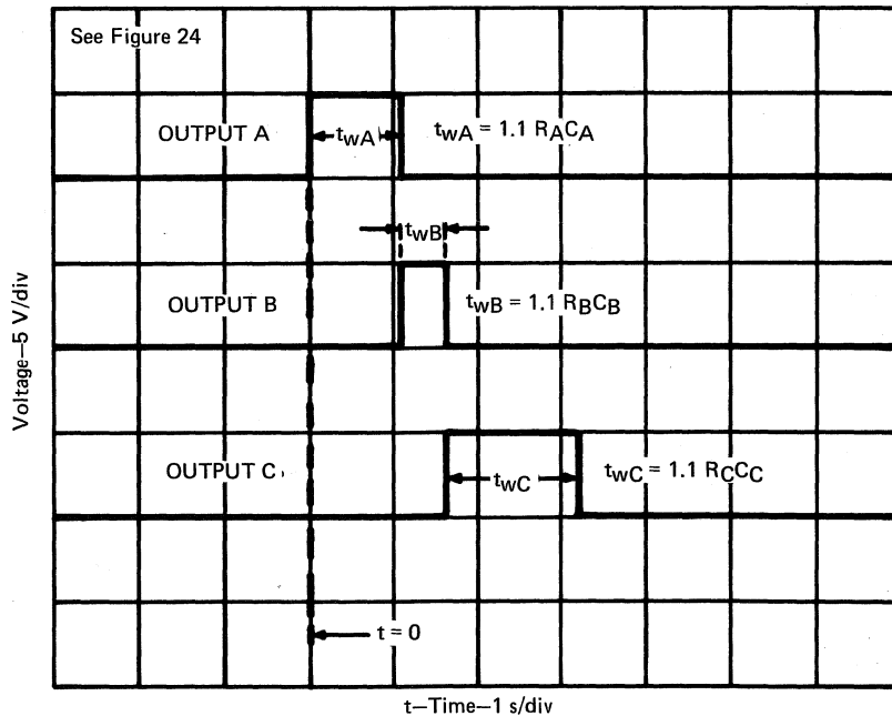
FIGURE 25—SEQUENTIAL TIMER WAVEFORMS
