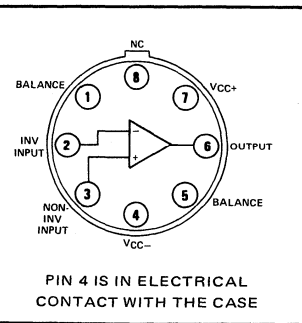
L PLUG-IN PACKAGE (TOP VIEW)
