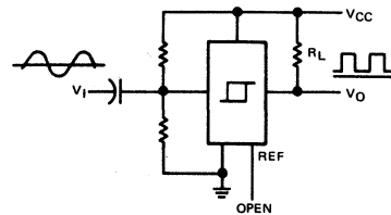
FIGURE 17—SINE-WAVE-TO-SQUARE-WAVE CONVERTER
