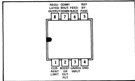
JG OR P DUAL-IN-LINE PACKAGE (TOP VIEW)
