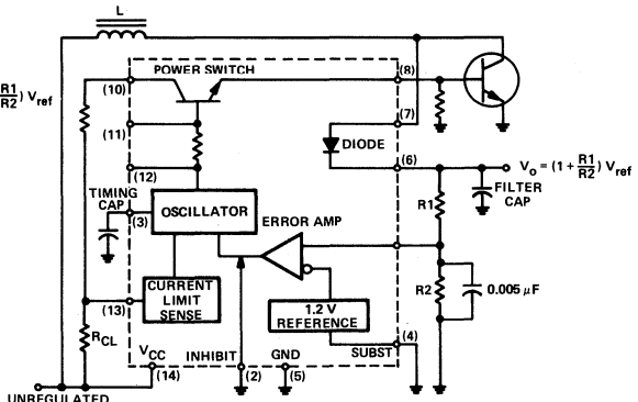
FIGURE 5—POSITIVE REGULATOR WITH BUFFERED OUTPUT
