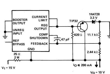
FIGURE 6—SHUNT REGULATOR
