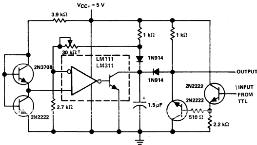
FIGURE 22—PRECISION SQUARER
