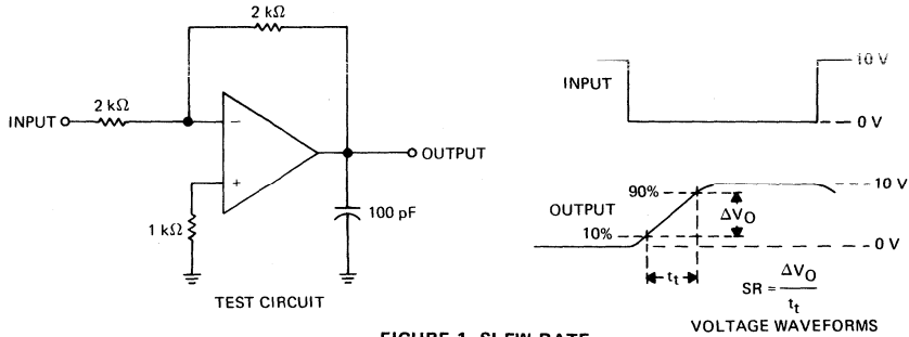
FIGURE 1—SLEW RATE
