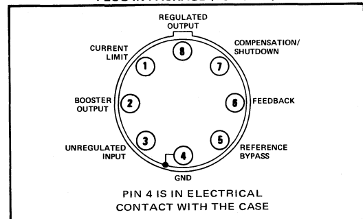
L PLUG-IN PACKAGE (TOP VIEW)
