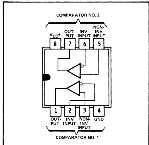
L PLUG-IN PACKAGE (TOP VIEW)
